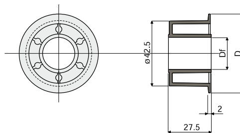
Roller for chain return (with flange)
