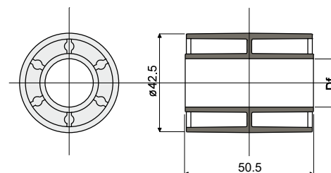
Double roller for chain return (without flange)
